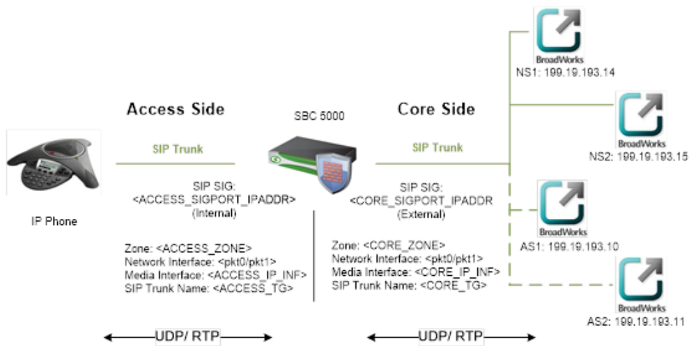
Figure 2: Reference Configuration
